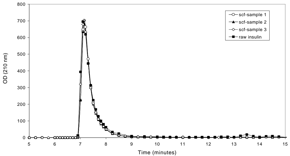
Figure 6 : HPLC Chromatograph of insulin samples after emulsion drying
